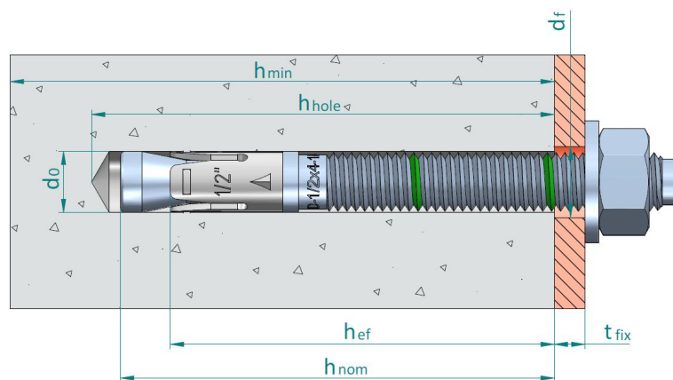
FIGURE 1—ANCHOR DIMENSIONS
